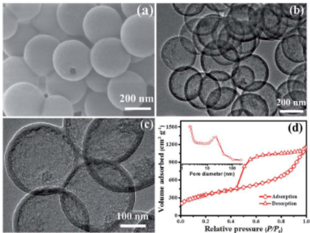
Typical SEM Image of ACS Material Hollow Carbon Spheres
