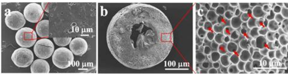
Typical SEM Image of ACS Material Large Size Mesoporous Carbon Spheres
