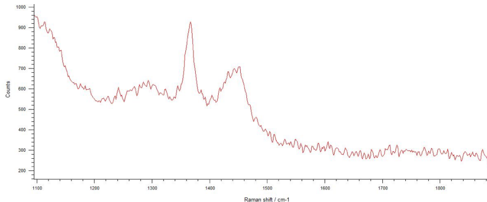
Typical Raman Spectrum of ACS Material Monolayer TTh-BN
