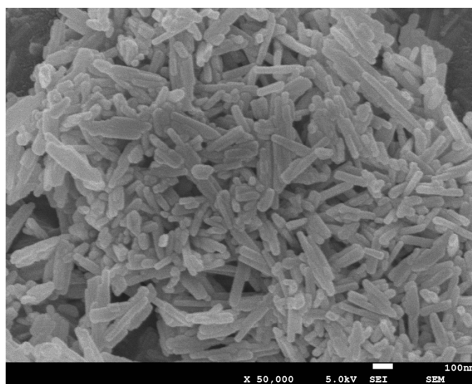
Typical SEM Image of ACS Material ZSM-23
