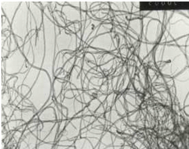
TEM Image of ACS Material Purified MWNTs-COOH (Length = 10-30 \mu\text{m} )
