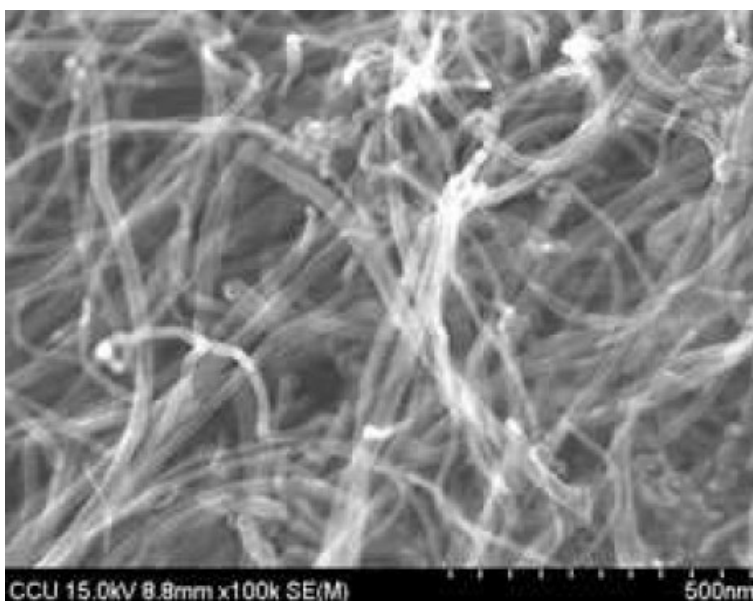
SEM Image of ACS Material Purified MWNTs-COOH (Length = 10-30 \mu\text{m} )
