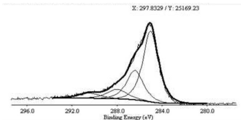
XPS Analysis of ACS Material Purified MWNTs-COOH (Length = 10-30 \mu\text{m} )
