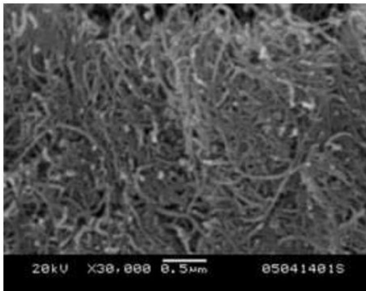
SEM Image of ACS Material Purified MWNTs-COOH (Length <10 \mu\text{m} )
