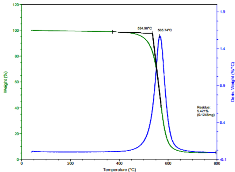
TG Analysis of ACS Material Purified SWCNTs-COOH (Length = 5-30 \mu\text{m} )
