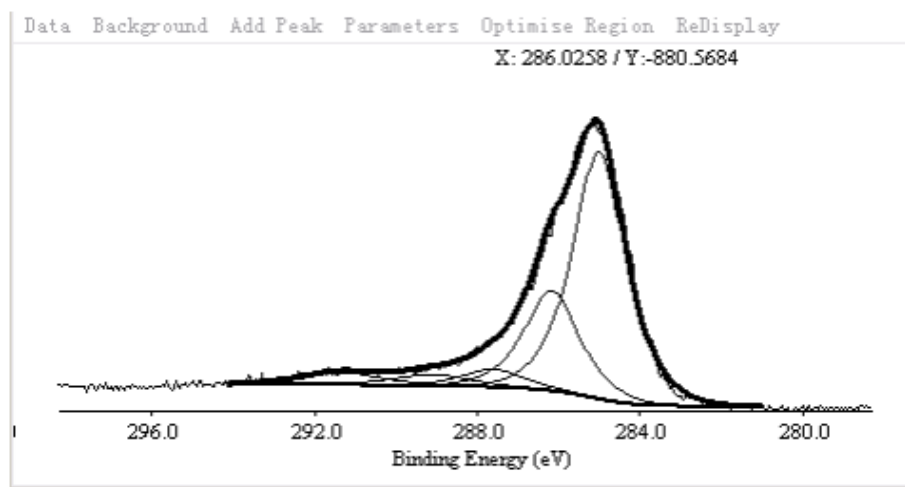
XPS Spectrum of ACS Material Purified SWCNTs-COOH (Length = 5-30 μm)
