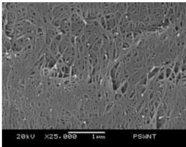
SEM Image of ACS Material Purified SWCNTs-COOH (Length = 5-30 μm)
