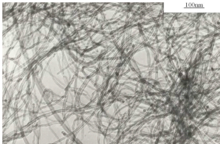
TEM Image of ACS Material Purified MWNTs-OH (Length = 10-30 \mu\text{m} )
