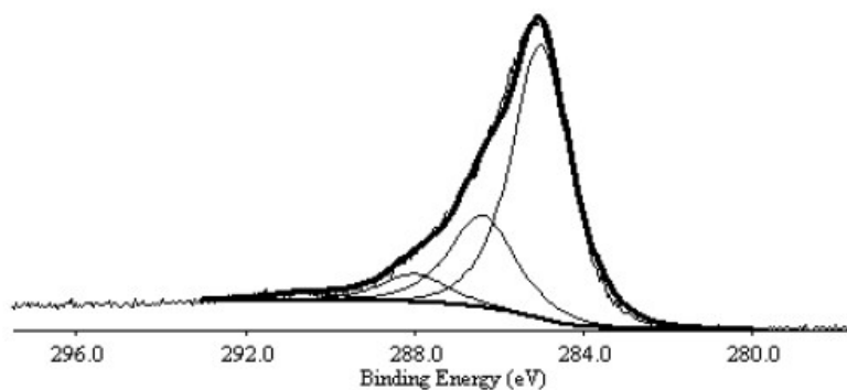
XPS Analysis of ACS Material Purified MWNTs-OH (Length = 10-30 \mu\text{m} )
