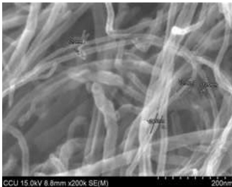
SEM Image of ACS Material Purified MWNTs (Length = 10-30 \mu\text{m} )
