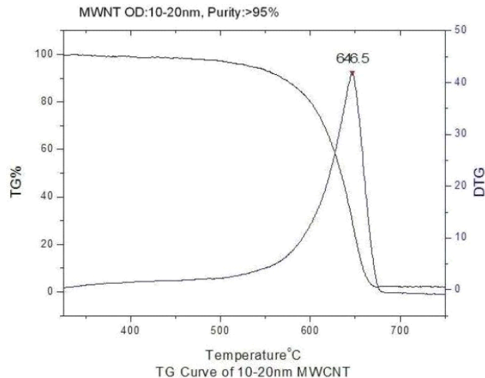
TG Curve of ACS Material Purified MWNTs (Length = 10-30 \mu\text{m} )
