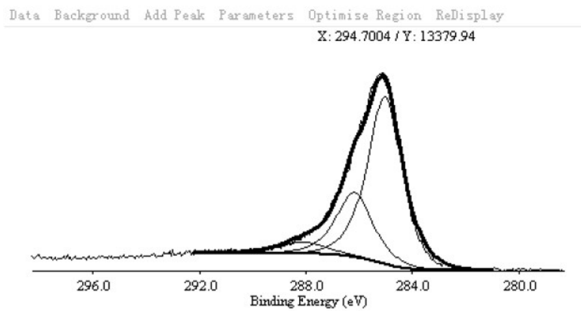
XPS Spectrum of ACS Material Purified MWNTs (Length = 10-30 \mu\text{m} )
