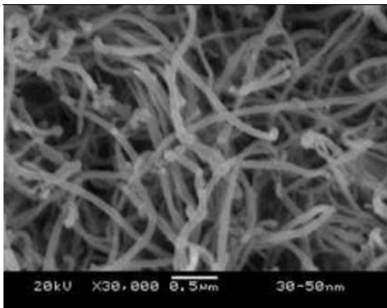
SEM Image (2) of ACS Material Purified MWNTs (Length <math><10 \mu\text{m}</math>)
