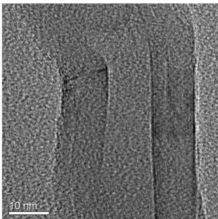
TEM Image of ACS Material Purified MWNTs (Length <math><10 \mu\text{m}</math>)
