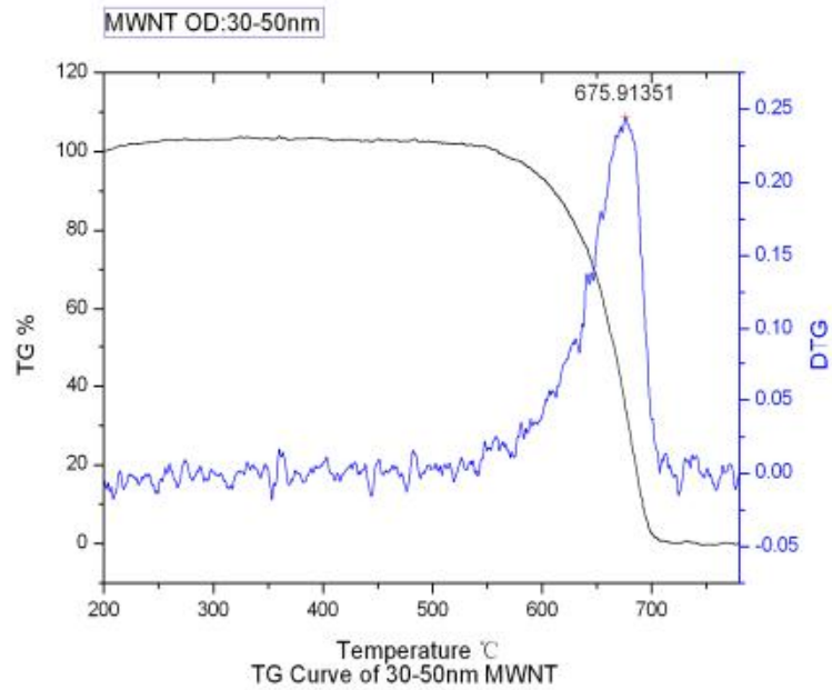
TG Curve of ACS Material Purified MWNTs (Length <math><10 \mu\text{m}</math>)
