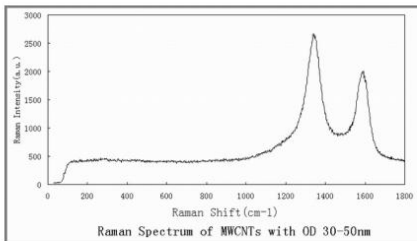
Raman Spectrum of ACS Material Purified MWNTs (Length <math><10 \mu\text{m}</math>)
